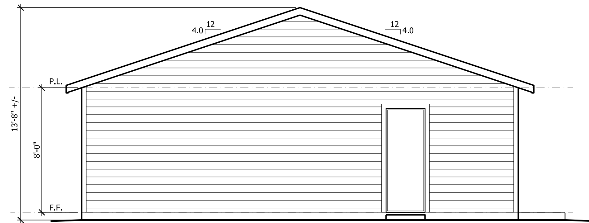
D LEFT ELEVATION 1 1/4" = 1'-0"
