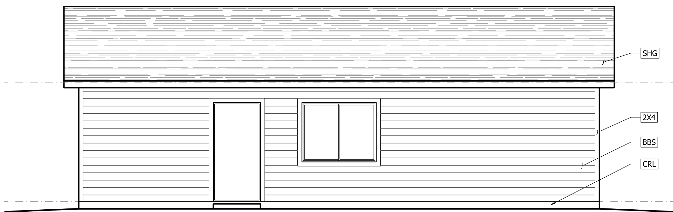
A FRONT ELEVATION 1 1/4" = 1'-0"
