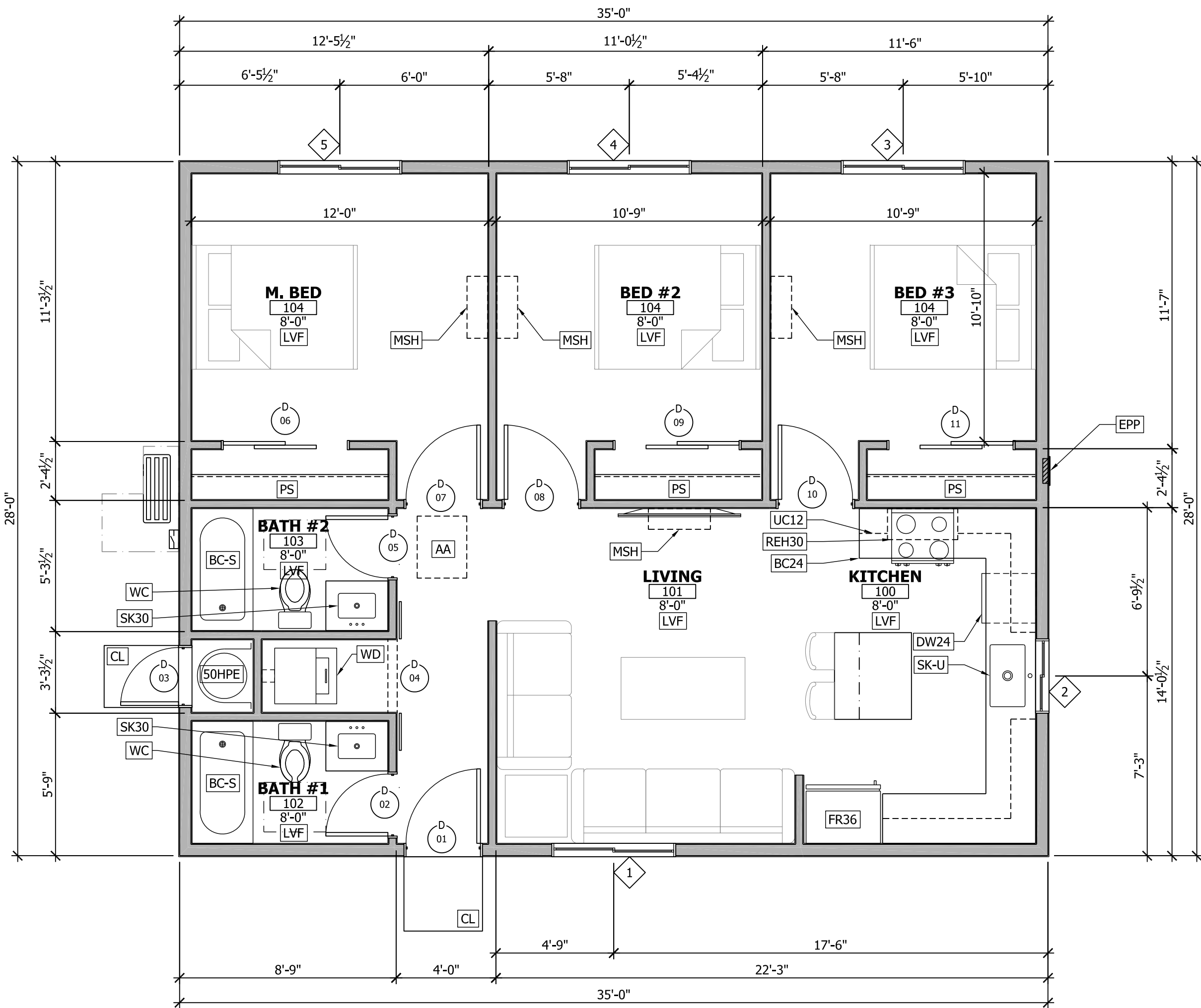
1 FLOOR PLAN 1 1/4" = 1'-0"
