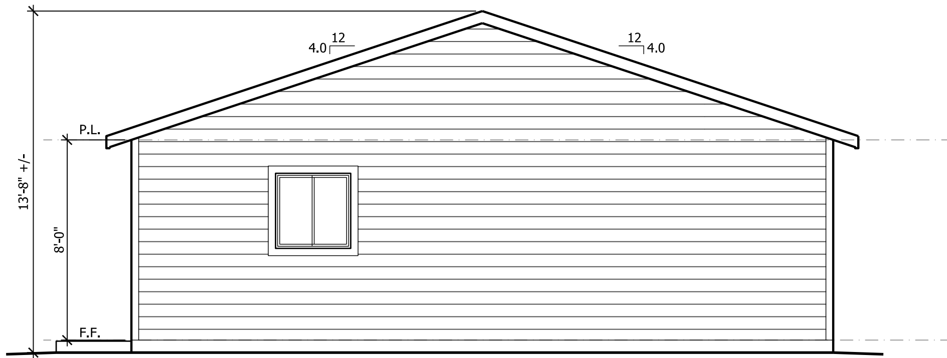
C RIGHT ELEVATION 1 1/4" = 1'-0"
